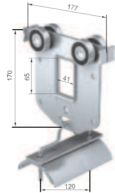
C63TT- Towing trolley
